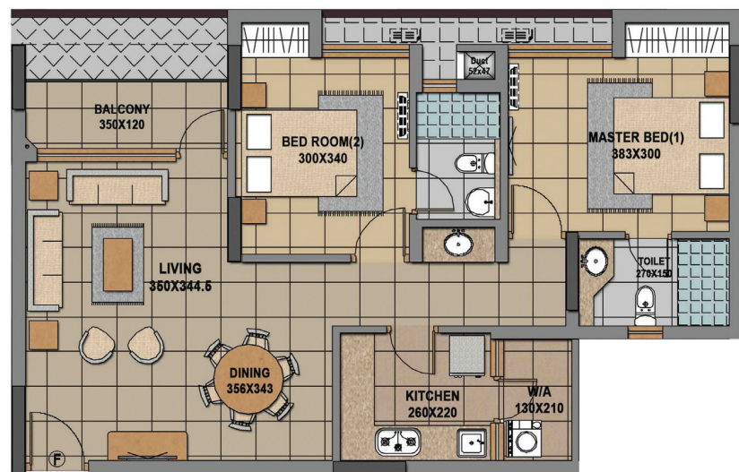
Unit - F, Area - 1113 Sq.ft
