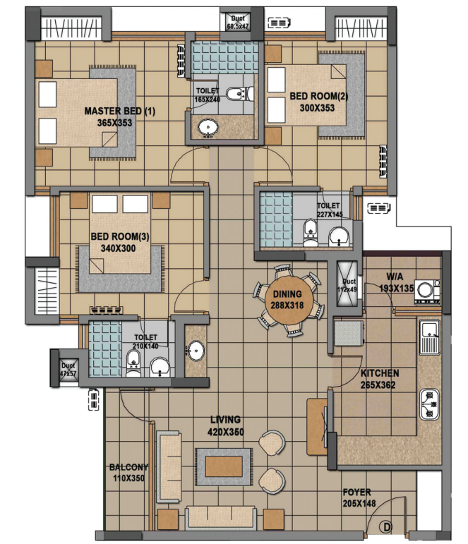
Unit - D, Area - 1449 Sq.ft
