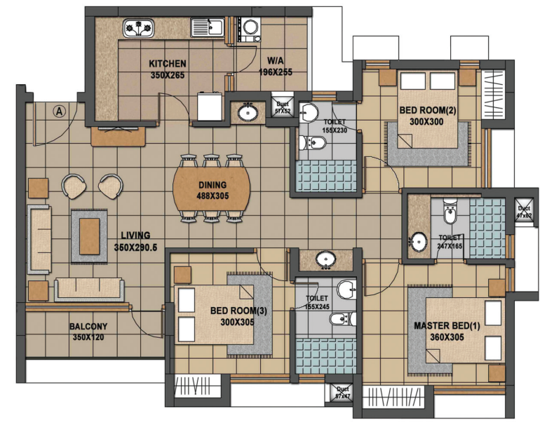
Unit - A, Area - 1394 Sq.ft
