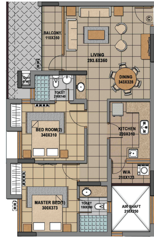
Unit - C, Area - 1085 Sq.ft
